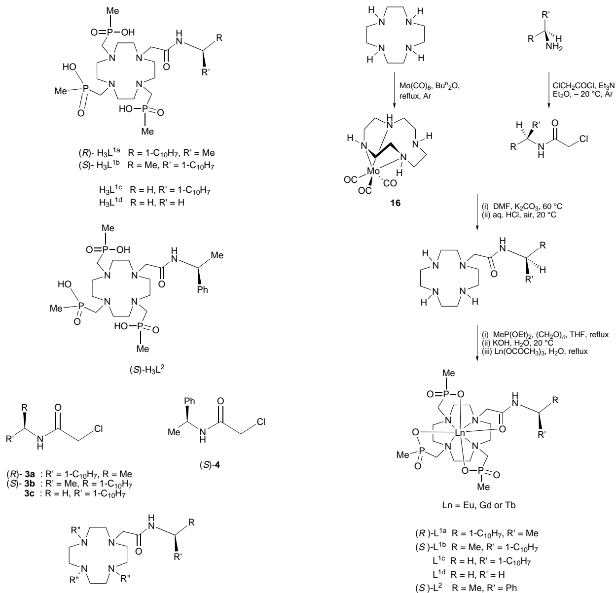
Scheme 1
